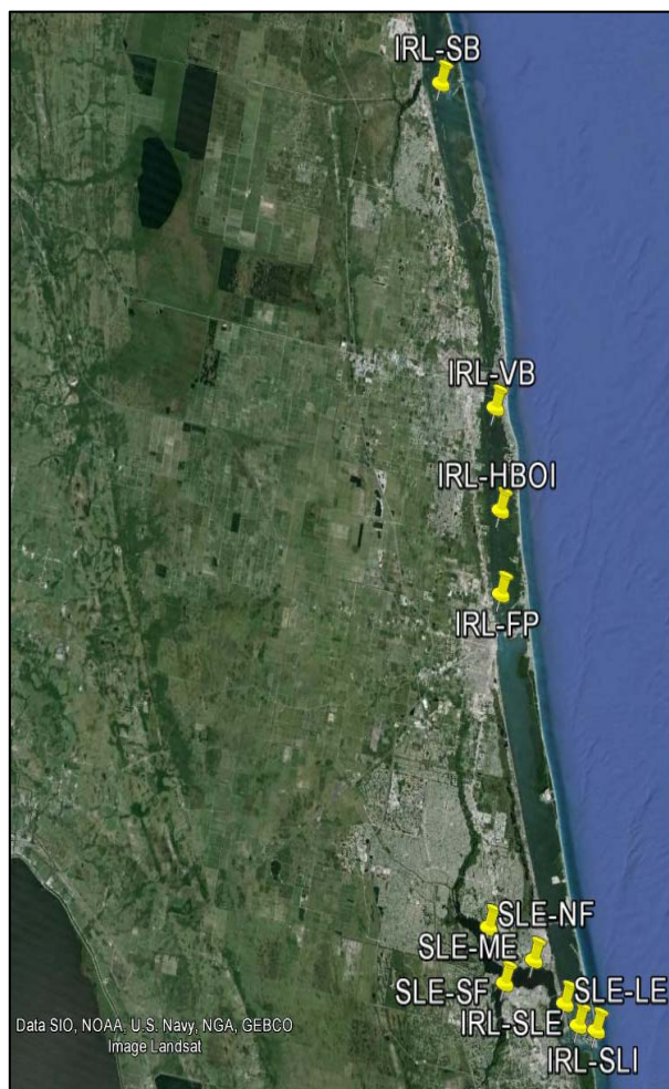
Figure 1. Strawman presented at the meeting for continuous LOBO monitoring in the IRL and SLE: IRL-SB (Sebastian), IRL-VB (Vero Beach), IRL-HBOI (Harbor Branch), IRL-FP (Fort Pierce), SLE-NF (North Fork), SLE-SF (South Fork), SLE-ME (Middle Estuary), SLE-LE (Lower Estuary Estuary), IRL-SLE (in the IRL near the confluence with the SLE), and IRL-SLI (IRL near St. Lucie Inlet).
