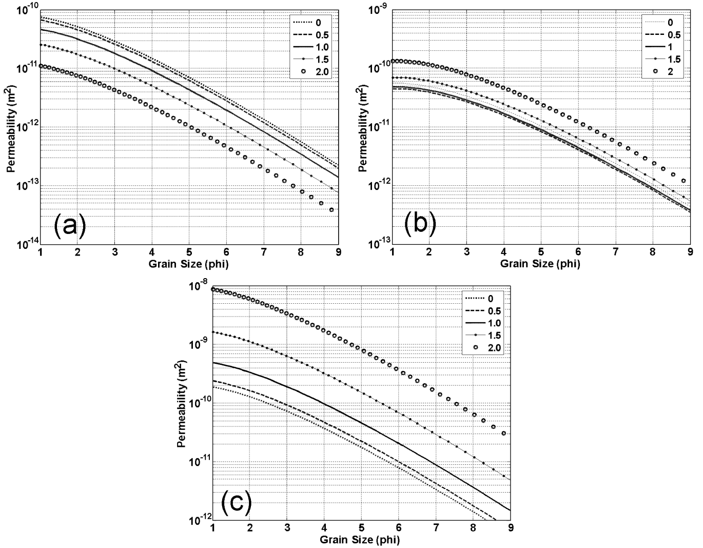
Fig. 4. Estimates of permeability from porosity and grain size for the following models. (a) Kozeny–Carman equation. (b) Interconnected pore model. (c) Parallel tube model. Permeability is plotted for log-normal pore- and grain-size distributions for five values of standard deviation: 0, 0.5, 1.0, 1.5, 2.0 \phi .
