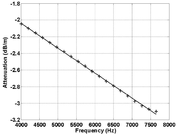
Fig. 19. Spectral ratio of echoes from the sediment-water interface and reflector D divided by the two-way path length. A line is fitted through the data by minimizing the square error. The slope of the line is 0.300 dB/m/kHz.
