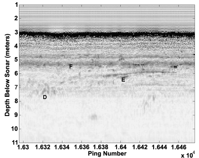
Fig. 18. Chirp sonar reflection profile at SAX-99 site. The vertical scale is based on a water sound speed of 1530 m/s. Attenuation rolloff is measured using reflector D. Reflectors E and F cannot be used for attenuation rolloff measurements, because the echoes contain interference caused by closely spaced reflectors (E) and a scattering layer (F).
