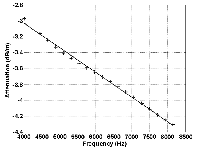
Fig. 14. Spectral ratio of echoes from the sediment-water interface and reflector A divided by the two-way path length. A line is fitted through the data by minimizing the square error. The slope of the line is 0.311 dB/m/kHz, the attenuation rolloff.
