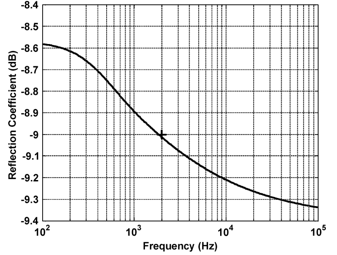
Fig. 22. Reflection coefficient as a function of frequency determined from inversion of chirp sonar data collected at the SAX-99 site. The + marks the reflection coefficient measurement of -9.0 dB at 2 kHz.
