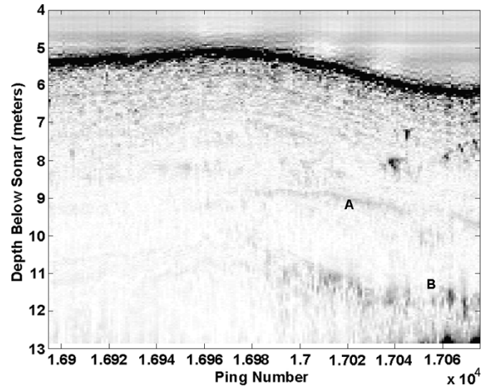
Fig. 13. Chirp sonar reflection profile at the SAX-99 site. The vertical scale is based on a water sound speed of 1530 m/s. Attenuation rolloff is measured using reflectors A and B.
