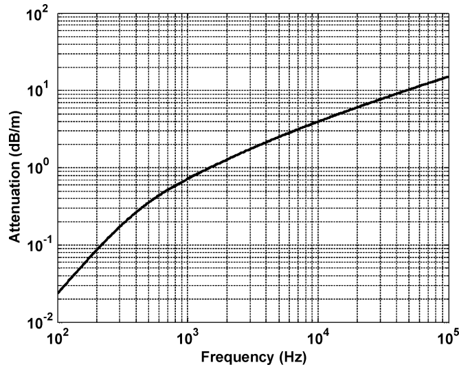
Fig. 24. Attenuation as a function of frequency determined from inversion of chirp sonar data collected at the SAX-99 site. This curve agrees with the attenuation function determined by Williams [4], who fits Biot model outputs to physical property data and in situ fast wave attenuation and velocity measurements collected at the SAX-99 site.
