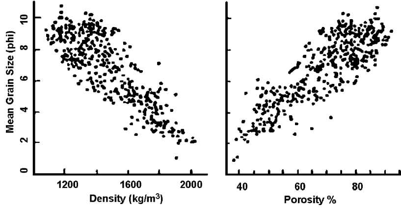
Fig. 2. Mean grain size \phi versus bulk density and porosity for sediment samples from the abyssal plain, abyssal hill, and continental shelf and slope [10].
