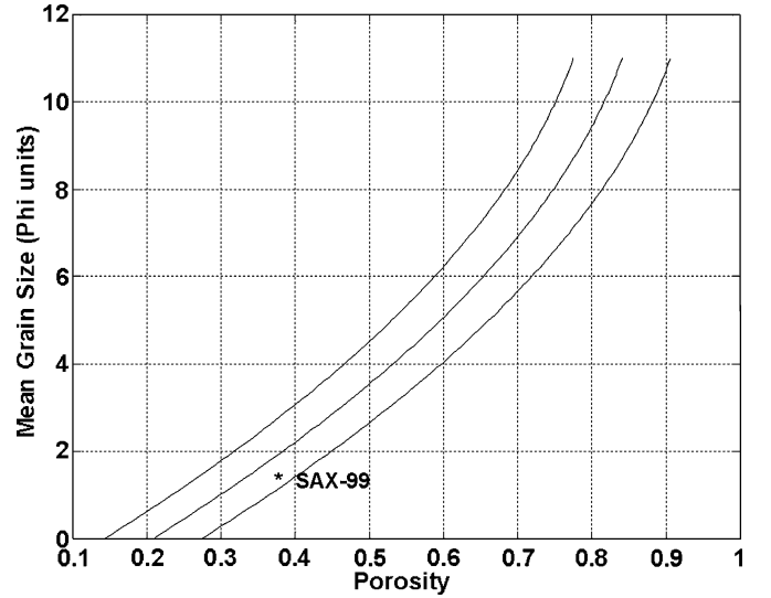
Fig. 3. Expected mean grain size plotted against porosity showing the 70% confidence limits of equation (33). The datum 1.32 \phi , n = 0.372 represents the average values of mean grain size and porosity of surficial sediments (top 13 cm) measured at the SAX-99 site off Fort Walton Beach, FL [13].
