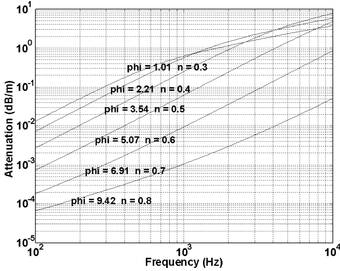
Fig. 7. Attenuation functions for six porosities and associated expected mean grain sizes for sediments from all environments. Note that slope of the attenuation function changes with frequency.
