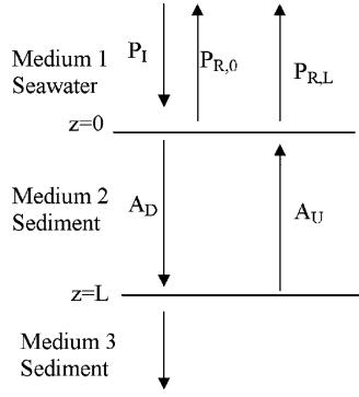
Fig. 10. Geometry for the discussion on estimating the slope of the attenuation function from the attenuation rolloff measurement.
