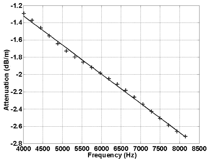
Fig. 15. Spectral ratio of echoes from the sediment–water interface and reflector B divided by the two-way path length. A line is fitted through the data by minimizing the square error. The slope of the line is 0.338 dB/m/kHz, the attenuation rolloff.
