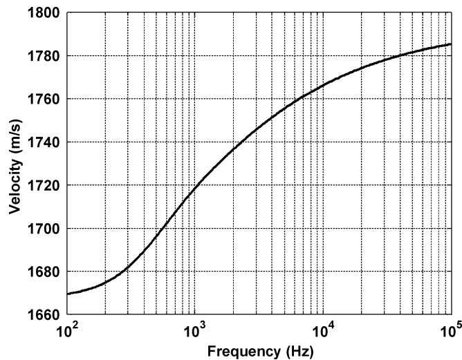
Fig. 25. Fast wave velocity as a function of frequency determined from inversion of chirp sonar data collected at the SAX-99 site. This curve agrees with the sound-speed function reported by Williams [4], who fits Biot model outputs to physical property data and in situ fast wave attenuation and velocity measurements collected at the SAX-99 site.
