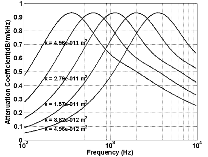
Fig. 9. Attenuation rolloff for the range of permeabilities expected for a sediment with a porosity of 0.389 and a mean grain size of 2.07\phi . At the attenuation rolloff measurement frequency of 6 kHz, the permeability can be uniquely determined from the attenuation rolloff.
