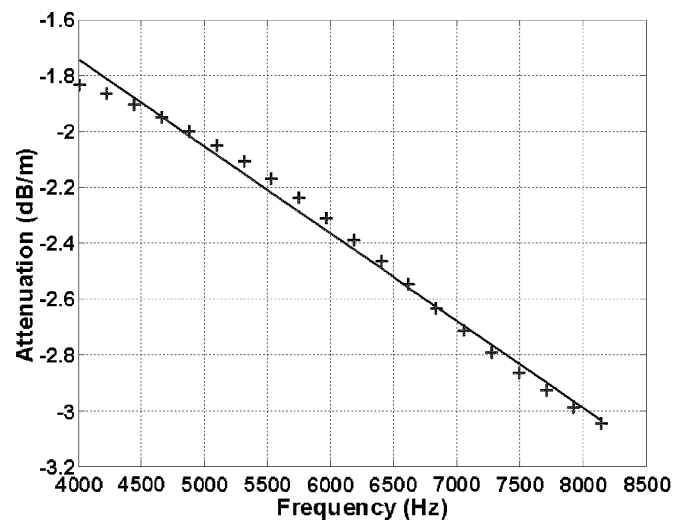
Fig. 17. Spectral ratio of echoes from the sediment–water interface and reflector C divided by the two-way path length. A line is fitted through the data by minimizing the square error. The slope of the line is 0.312 dB/m/kHz, the attenuation rolloff.
