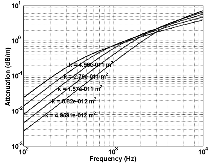
Fig. 8. Fast wave attenuation for the range of permeabilities expected for a sediment with a porosity of 0.389 and a mean grain size of 2.07\phi .
