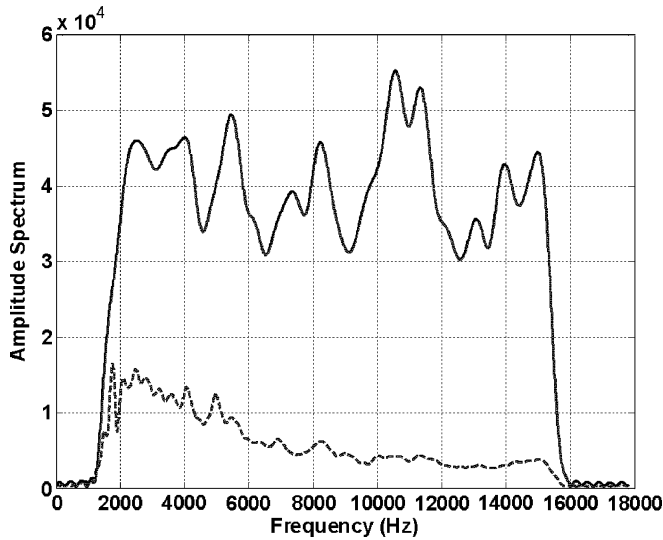
Fig. 12. Amplitude spectra of one air-water interface echo (collected at calibration site: solid line) and one sand-water interface echo (collected at SAX-99 site: dashed line).
