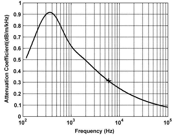
Fig. 23. Attenuation coefficient as a function of frequency determined from on inversion of chirp sonar data collected at the SAX-99 site. The + marks the attenuation rolloff measurement of 0.3155 dB/m/kHz at a center frequency of 6 kHz.
