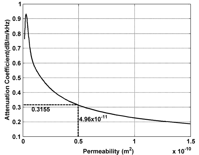
Fig. 21. Attenuation rolloff as a function of permeability at 6 kHz for sediments with a porosity of 0.389. The first iteration of the inversion predicts a permeability 4.96 \times 10^{-11} \text{ m}^2 for SAX-99 site sediments.
