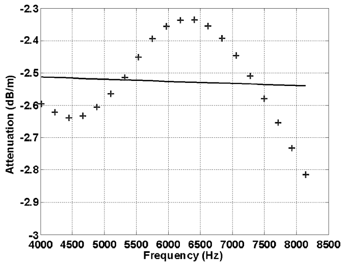
Fig. 20. Spectral ratio of the echoes from Reflector E and the sediment water interface contains interference from echoes originating at the top and bottom of the thin layer at reflector E shown in Fig. 18. Oscillations in the spectral ratio indicate interfering echoes.
