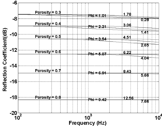
Fig. 5. Reflection coefficient function of frequency for six values of porosity. For each value of porosity, the reflection coefficient function is plotted for the expected mean grain size and for the 70% confidence intervals. The expected grain size introduces only a small error into the estimation of porosity from the reflection coefficient for most surficial sediments.
