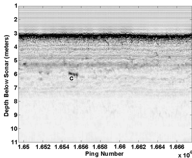
Fig. 16. Chirp sonar reflection profile at the SAX-99 site. The vertical scale is based on a water sound speed of 1530 m/s. Attenuation rolloff is measured using reflector C.
